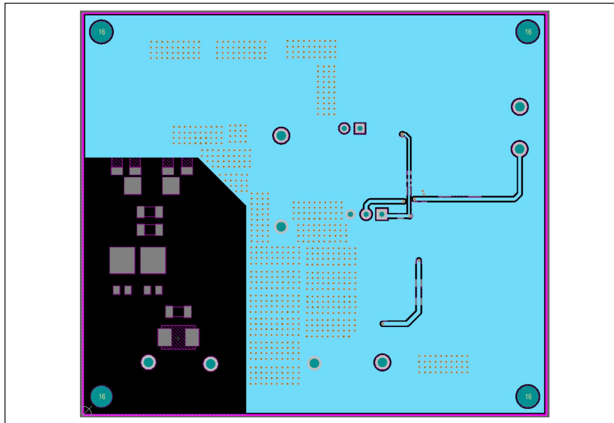
Figure 6 Board PCB Layout - Mid-Layer 2
