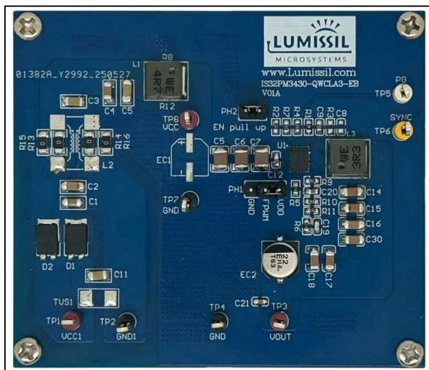
Figure 1 Photo of IS32PM3430 Evaluation Board
