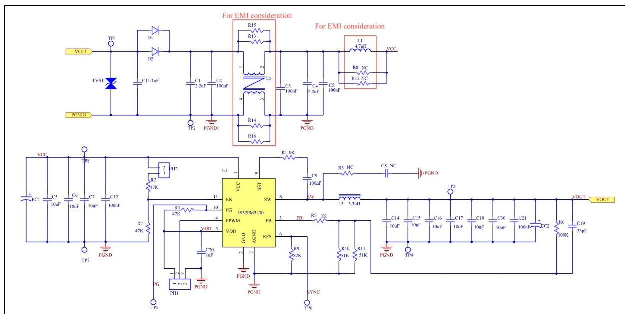
Figure 3 IS32PM3430 Demo Board Schematic
