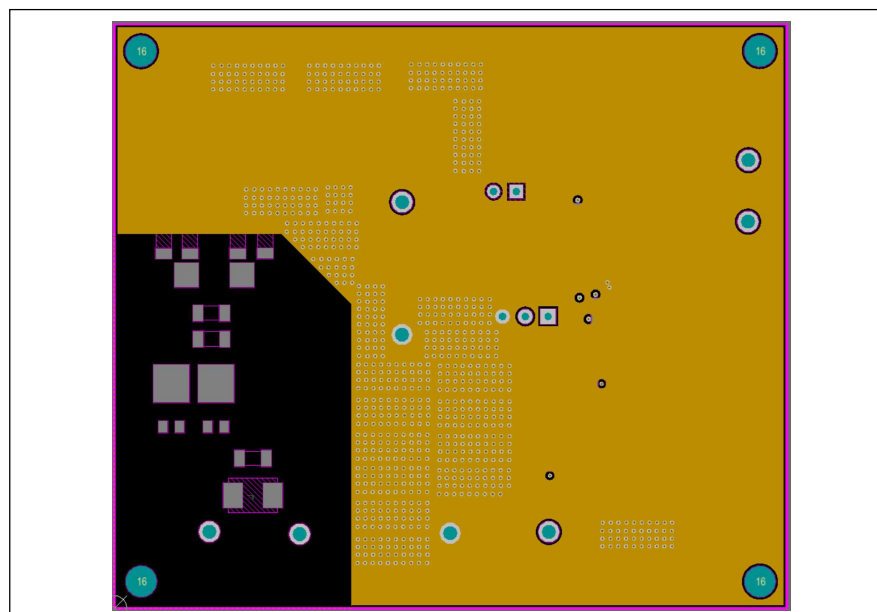
Figure 5 Board PCB Layout - Mid-Layer 1
