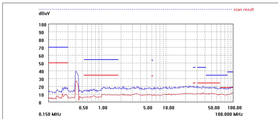
Figure 9 CISPR-25 Class 5 Conducted EMI Scan (GND)
