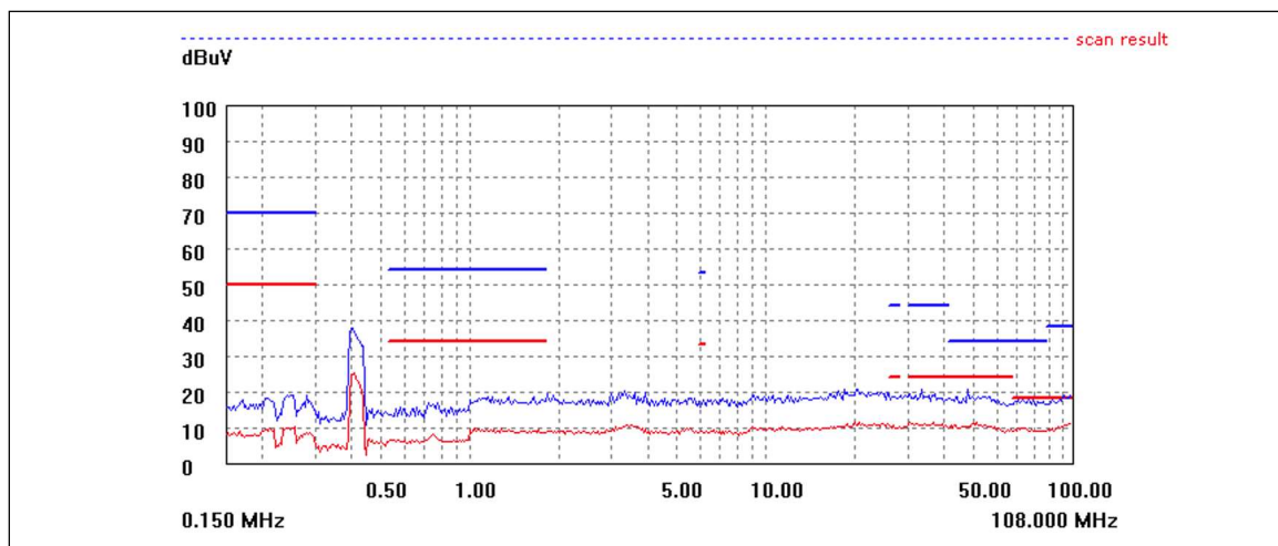
Figure 8 CISPR-25 Class 5 Conducted EMI Scan (VCC)
