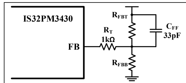
Figure 2 Feedback Network
