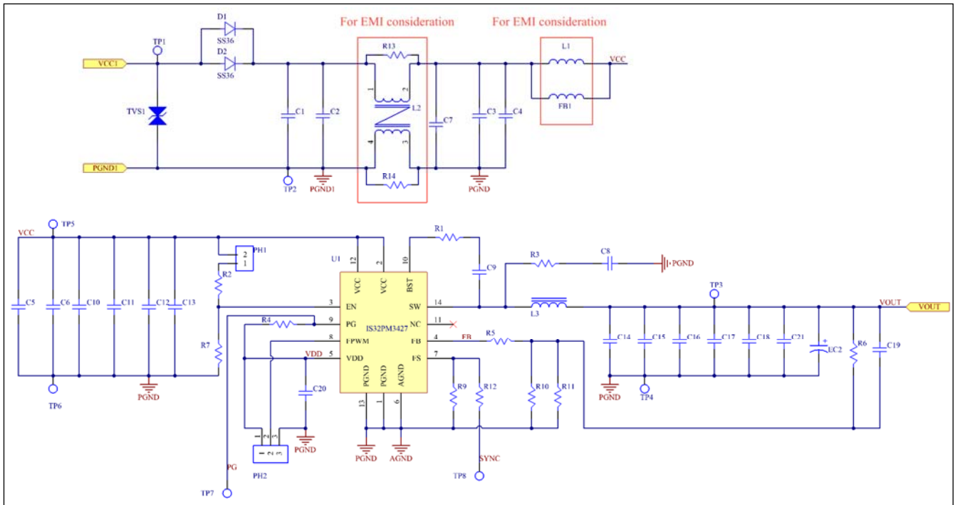
Figure 3 IS32PM3427 Demo Board Schematic
