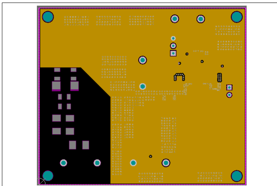
Figure 5 Board PCB Layout - Mid-Layer 1
