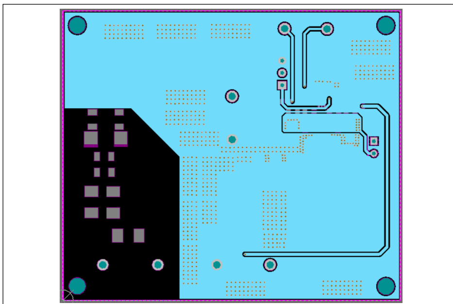
Figure 6 Board PCB Layout - Mid-Layer 2
