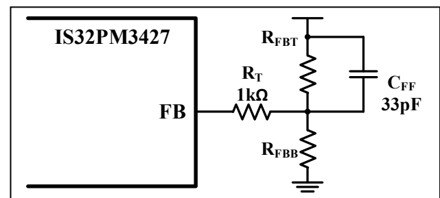
Figure 2 Feedback Network
