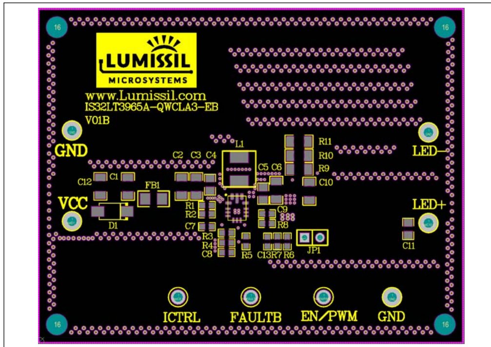
Figure 4 Board Component Placement Guide - Top Overlay
