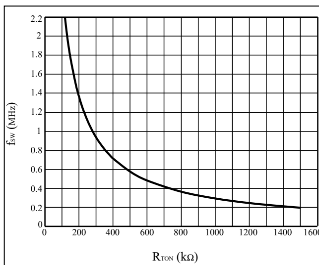
Figure 2 Operating Frequency vs. R_{TON} Resistance
