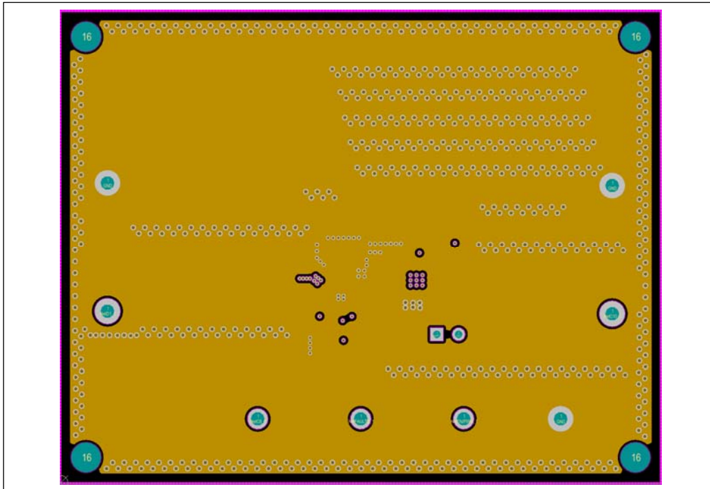
Figure 6 Board PCB Layout - Mid-Layer 1
