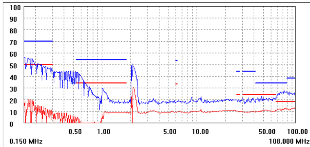
Figure 11 CISPR-25 Class 5 Conducted EMI Scan (VIN-)
