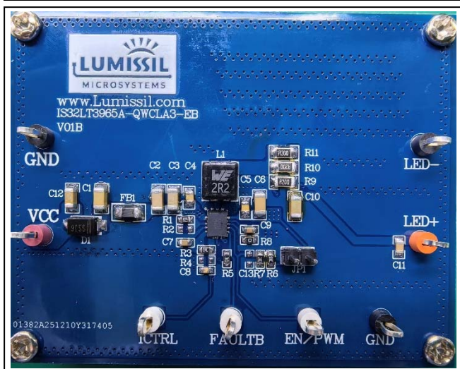
Figure 1 Photo of IS32LT3965A Evaluation Board
