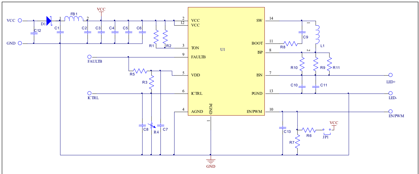
Figure 3 IS32LT3965A Demo Board Schematic
