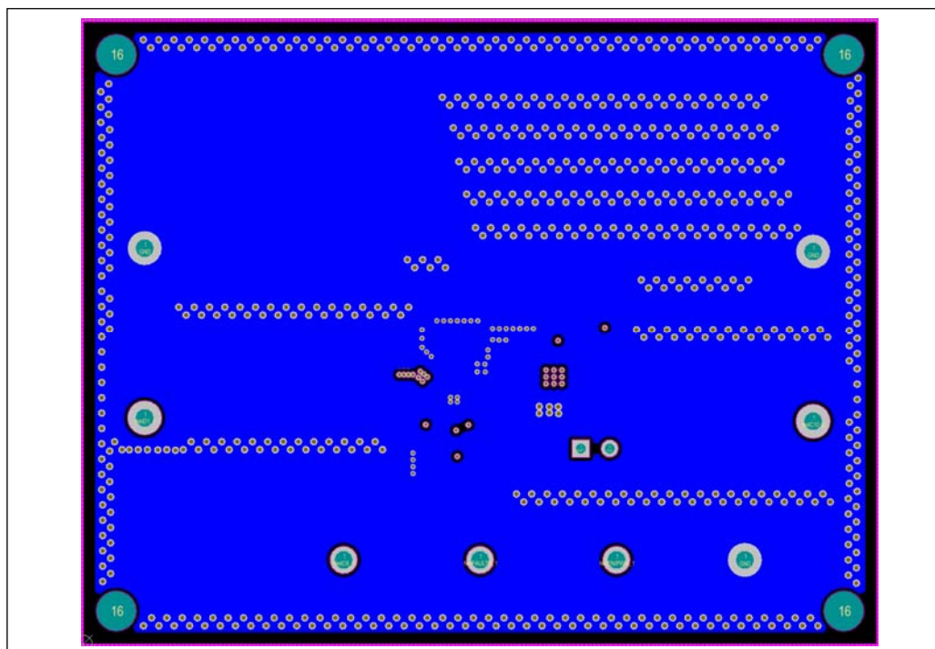
Figure 8 Board PCB Layout - Bottom Layer
