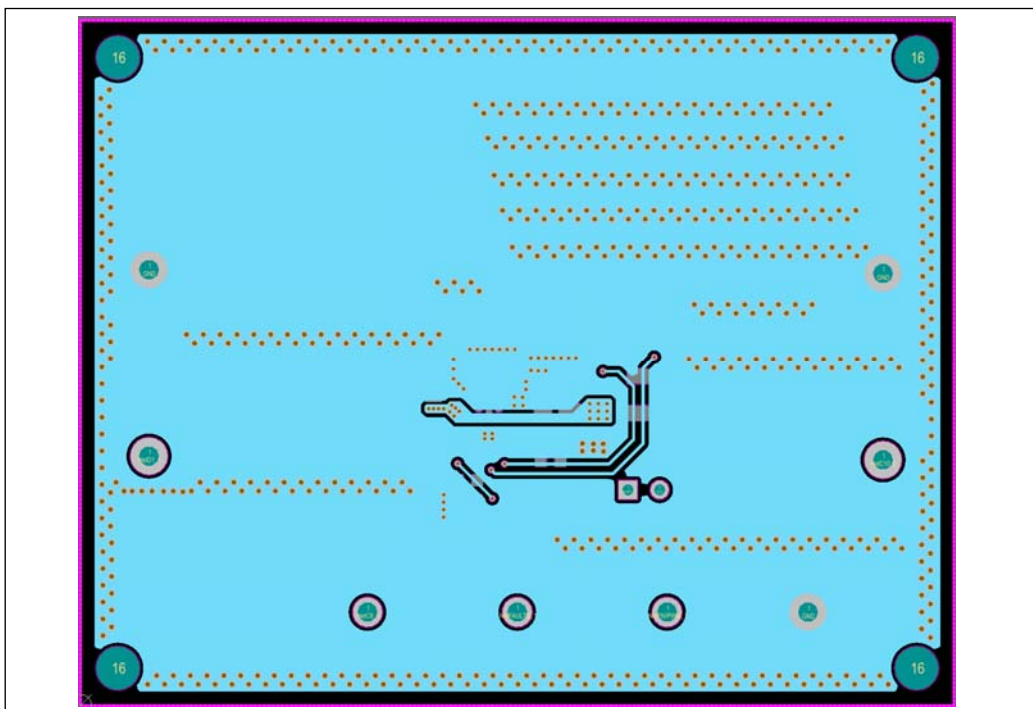
Figure 7 Board PCB Layout - Mid-Layer 2
