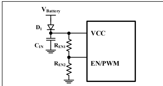
Figure 42 External UVLO for VCC
