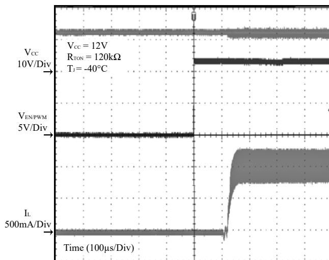
Figure 36 EN/PWM Enable ( I_{OUT} = 1A )
