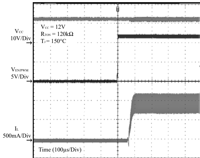
Figure 38 EN/PWM Enable ( I_{OUT} = 1\text{A} )
