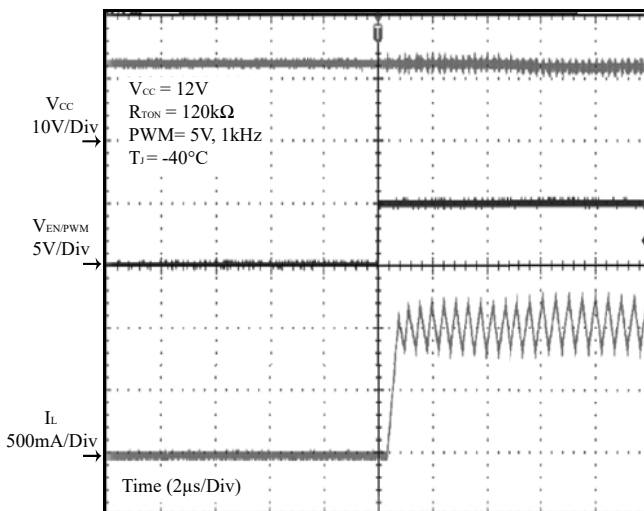
Figure 24 PWM On ( I_{OUT} = 1A )
