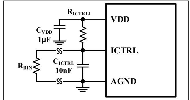
Figure 47 Analog Dimming For LED Binning
