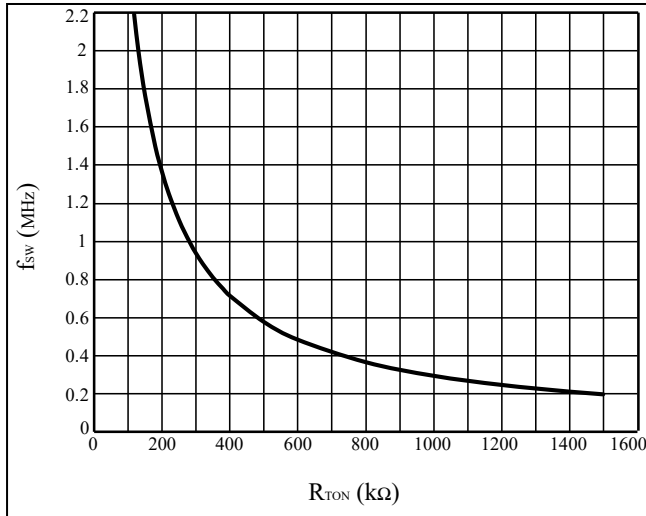
Figure 52 Operating Frequency vs. R_{TON} Resistance
