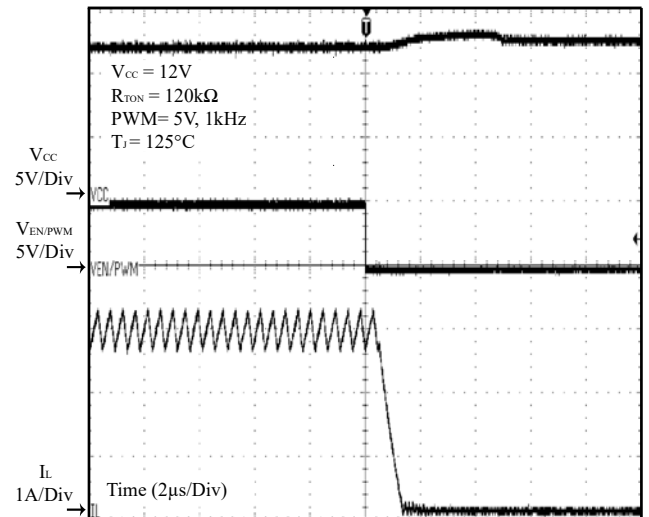
Figure 35 PWM Off ( I_{OUT} = 3A )
