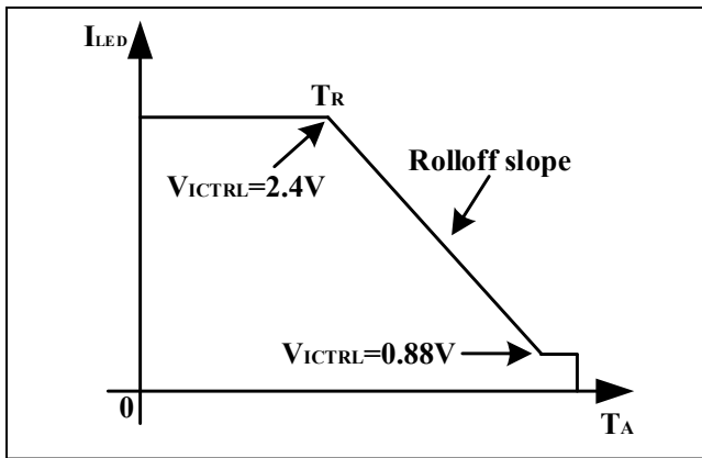
Figure 49 Analog Dimming For Thermal Roll-off Protection
