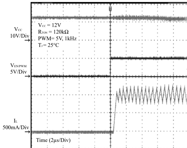
Figure 26 PWM On ( I_{OUT} = 1A )
