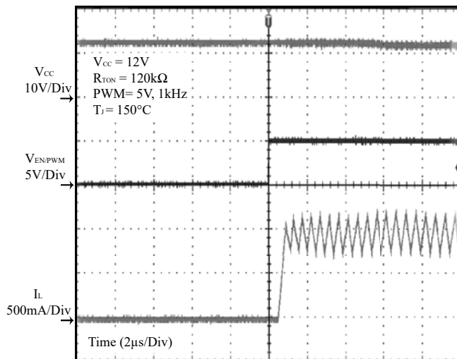
Figure 28 PWM On ( I_{OUT} = 1A )
