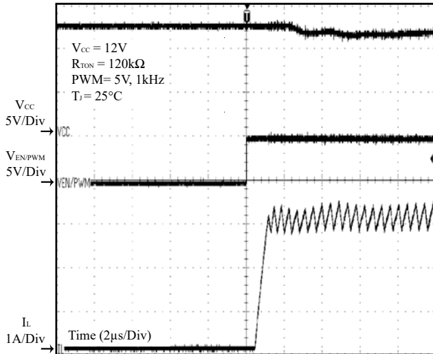
Figure 32 PWM On ( I_{OUT} = 3A )
