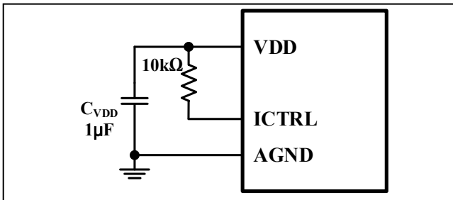
Figure 46 ICTRL Pin Unused
