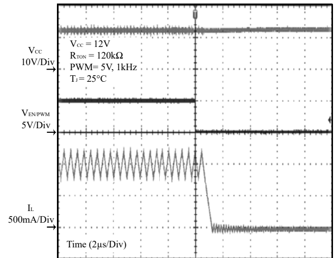
Figure 27 PWM Off ( I_{OUT} = 1A )
