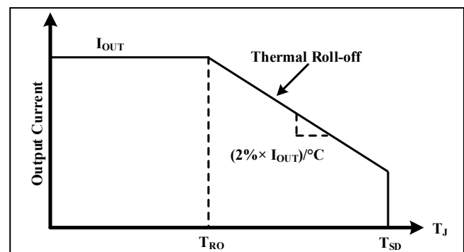
Figure 58 Thermal Roll-off
