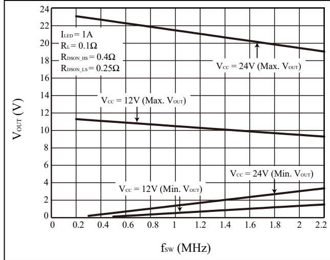
Figure 54 Minimum and Maximum Output Voltage versus Operating Frequency (minimum t_{ON} =80ns and minimum t_{OFF} =90ns)
