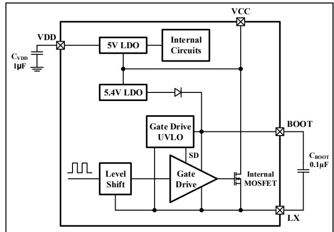
Figure 43 LDOs and Bootstrap Circuit
