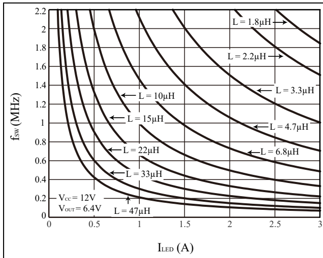
Figure 56 Inductance Selection Based On 30% Current Ripple
