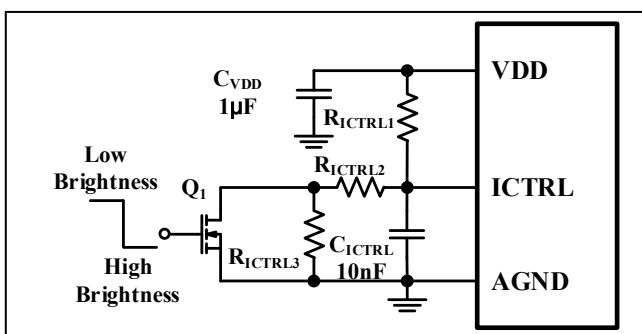
Figure 50 ICTRL Pin for Dual Brightness Output
