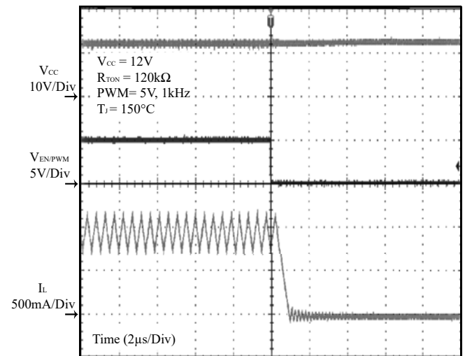
Figure 29 PWM Off ( I_{OUT} = 1A )
