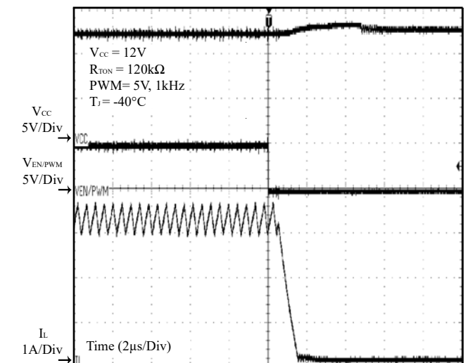
Figure 31 PWM Off ( I_{OUT} = 3A )
