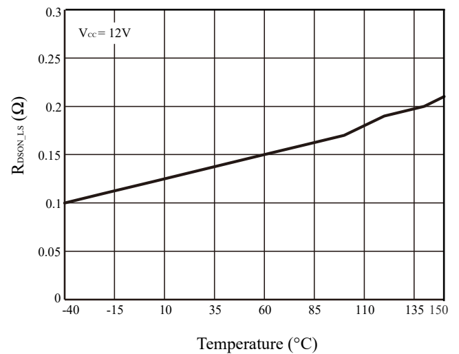
Figure 7 R_{DS(on)_LS} vs. Temperature
