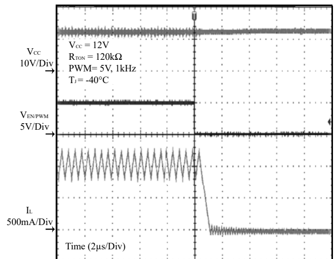
Figure 25 PWM Off ( I_{OUT} = 1A )
