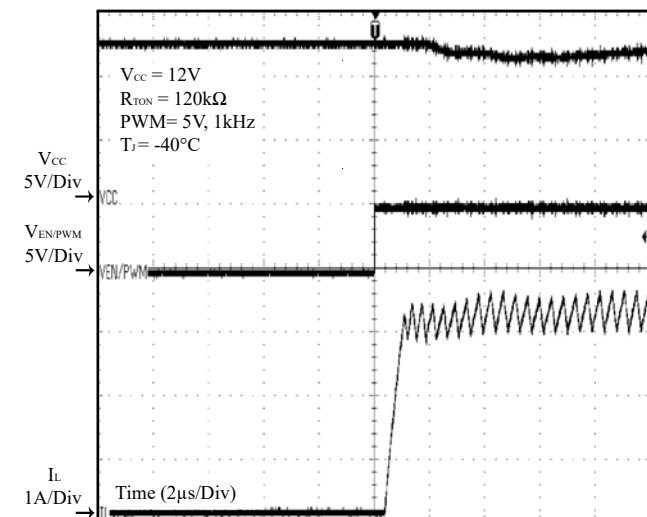
Figure 30 PWM On ( I_{OUT} = 3A )
