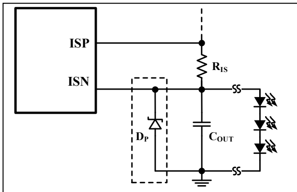
Figure 59 Schottky Diode for ISN/ISP Protection
