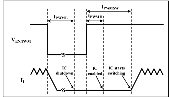
Figure 44 Device Shutdown and Enable
