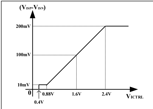
Figure 45 Analog Dimming Graph
