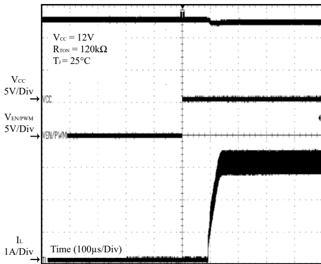
Figure 40 EN/PWM Enable ( I_{OUT} = 3\text{A} )
