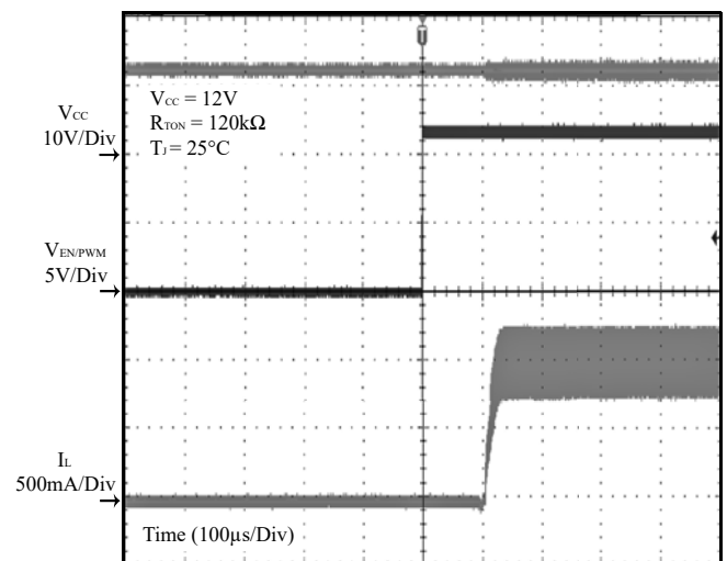
Figure 37 EN/PWM Enable ( I_{OUT} = 1A )
