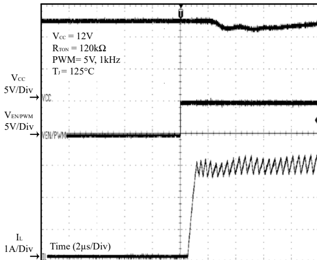
Figure 34 PWM On ( I_{OUT} = 3A )
