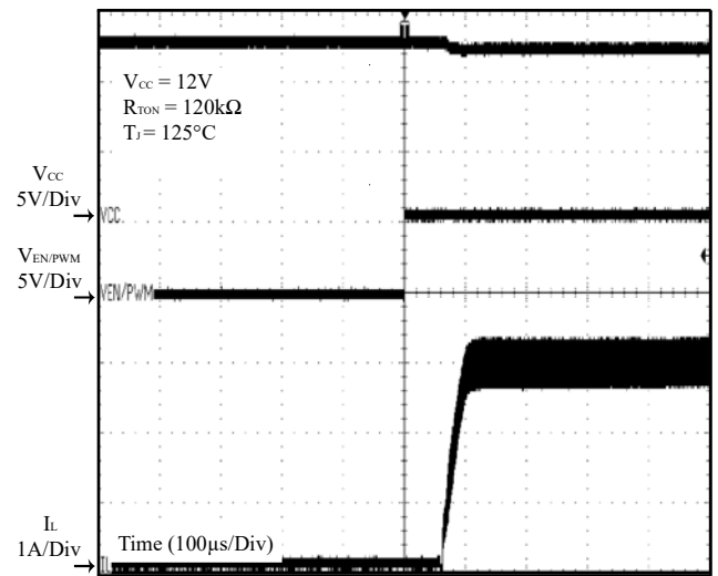
Figure 41 EN/PWM Enable ( I_{OUT} = 3\text{A} )
