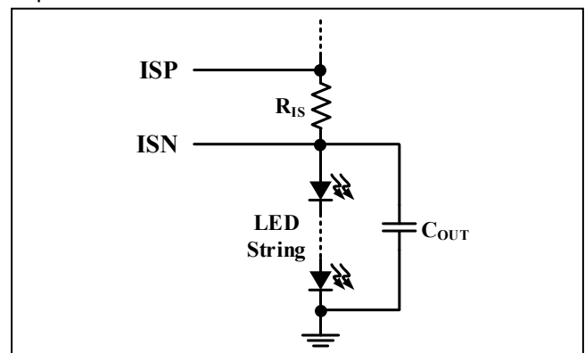
Figure 51 Output Capacitor Excluding R IS
