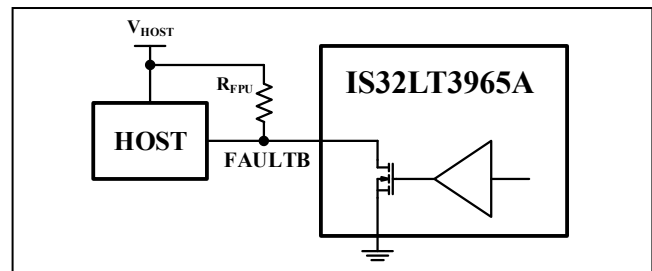
Figure 57 Host Monitors The Fault Reporting
