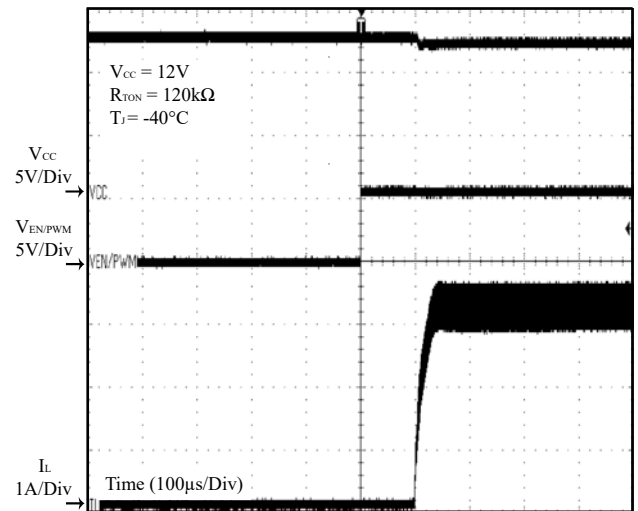
Figure 39 EN/PWM Enable ( I_{OUT} = 3\text{A} )
