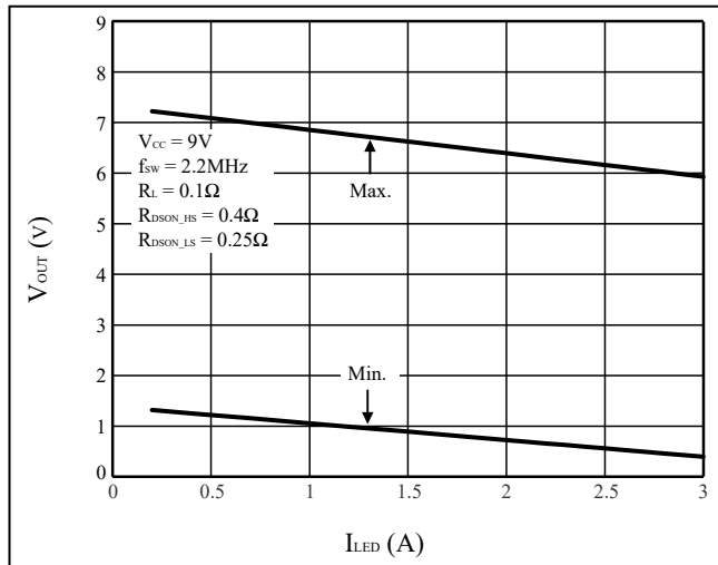
Figure 55 Minimum and Maximum Output Voltage versus LED Current (minimum t_{ON} =80ns and minimum t_{OFF} =90ns)
