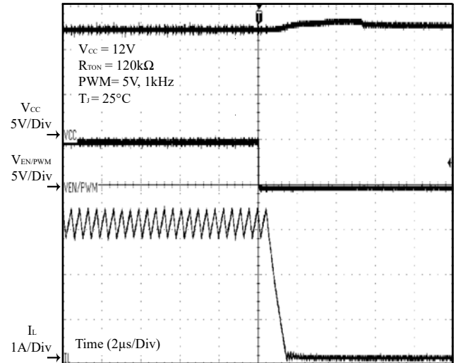
Figure 33 PWM Off ( I_{OUT} = 3A )
