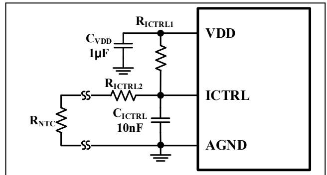
Figure 48 ICTRL Pin with NTC for Thermal Roll-off Protection
