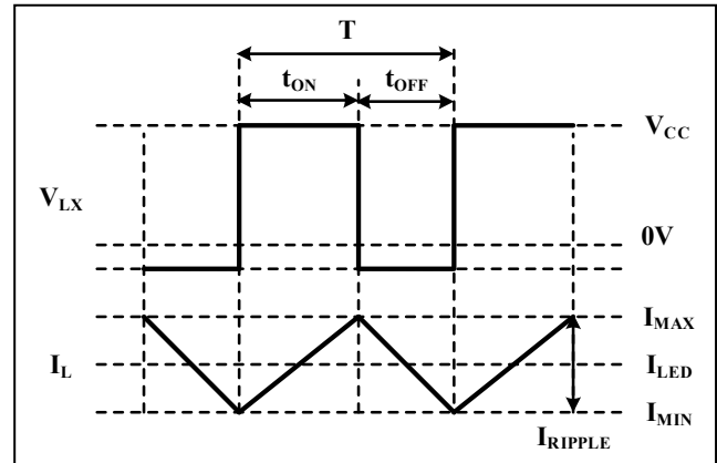
Figure 53 Operating Waveform
