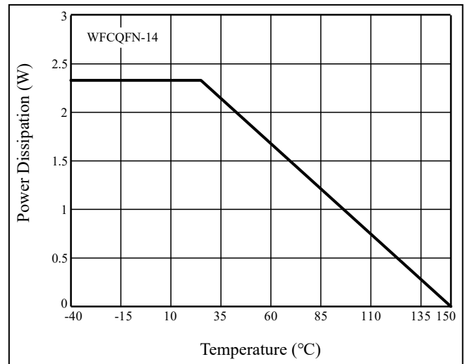
Figure 60 Dissipation Curve
