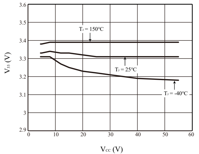
Figure 11 V_{33} vs. V_{CC}
