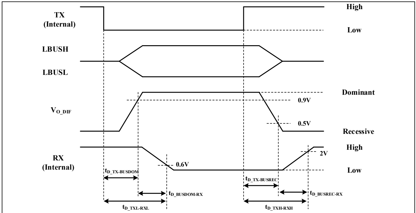
Figure 43 LumiBus Interface Timing
