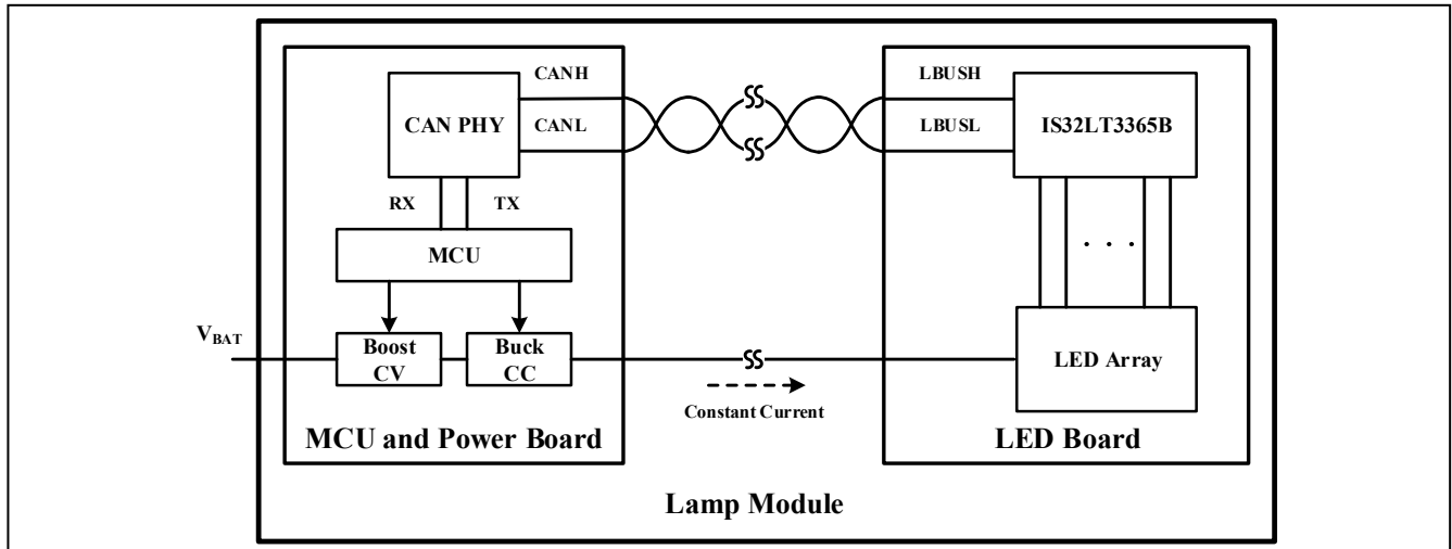
Figure 19 LumiBus Interface for Long Distance Intramodular Communication
