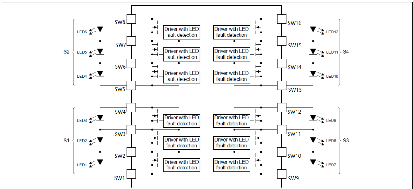
Figure 24 Bypass Switch Groups
