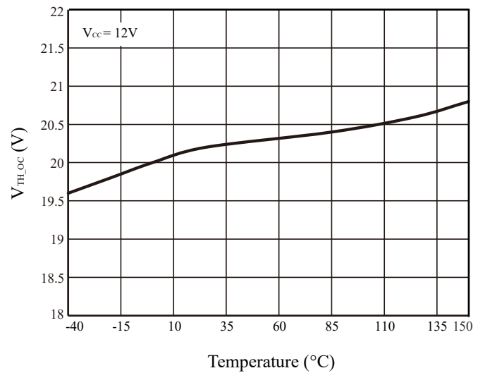
Figure 17 V_{TH\_OC} vs. Temperature
