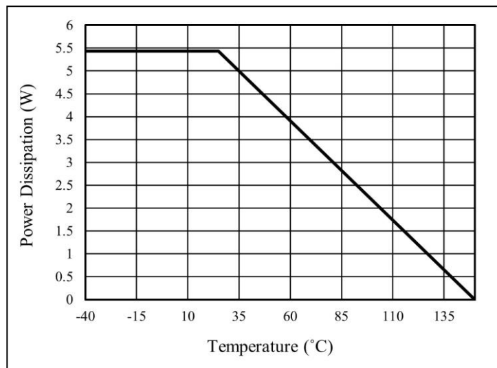
Figure 72 Dissipation Curve
