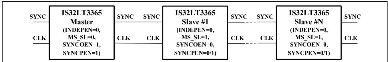
Figure 30 PWM Hardware Synchronization Connection
