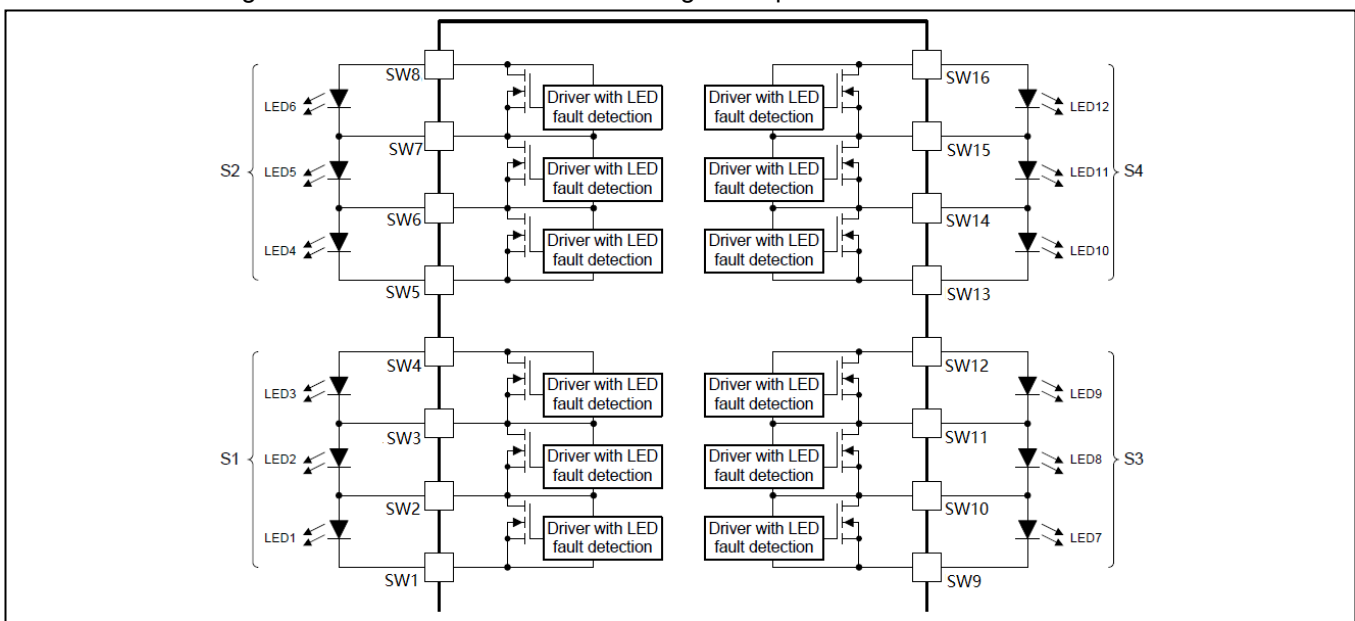
Figure 67 LED Sub-Strings
