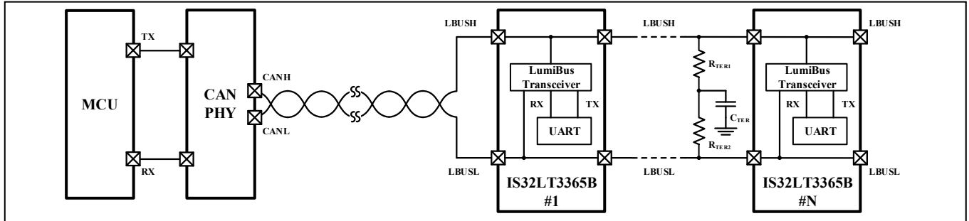
Figure 42 LumiBus Interface Connection
