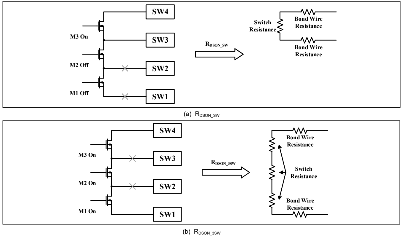
Figure 22 Bypass Switch On-resistance
