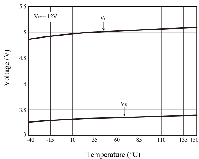
Figure 14 V_5 & V_{33} vs. Temperature
