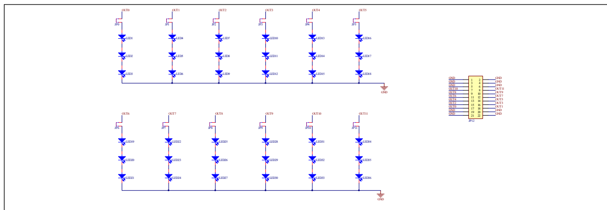
Figure 4: 18 channel LED Application Schematic
