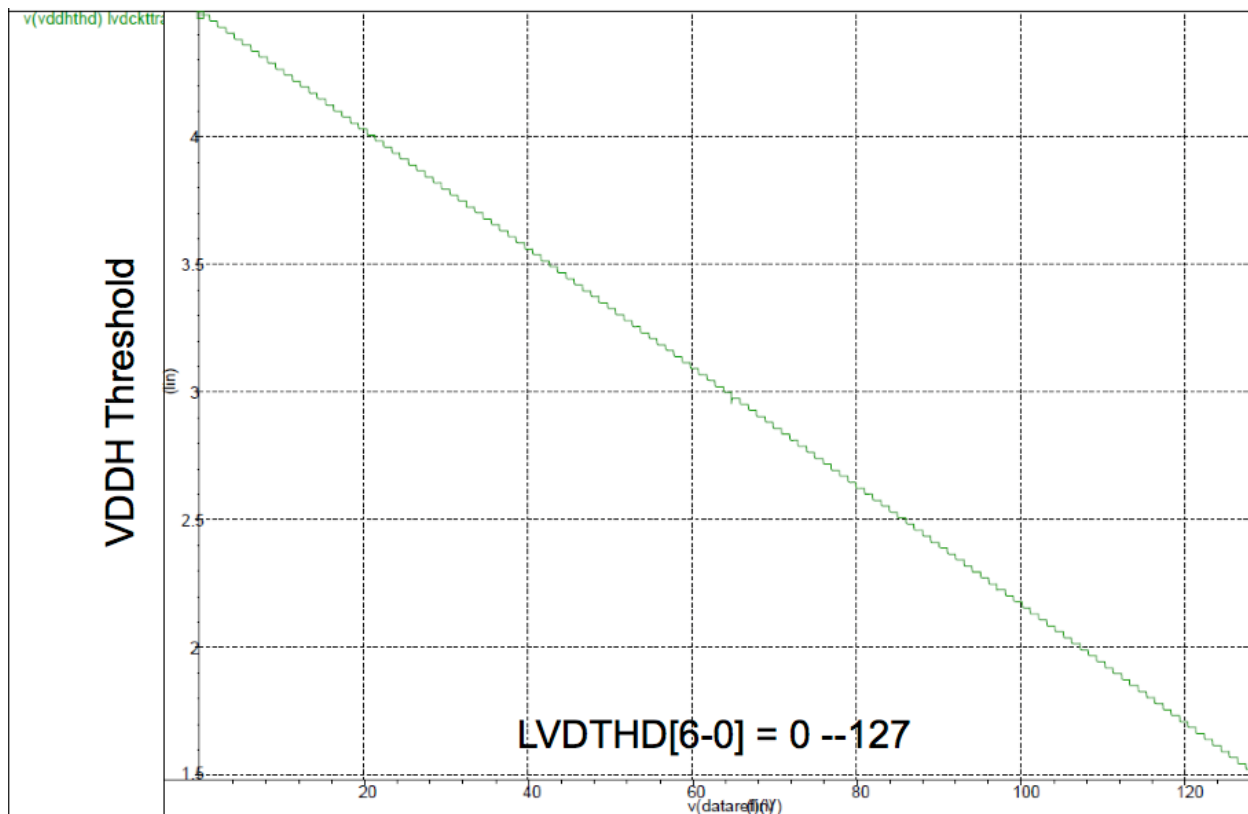
Figure 15-1 LVD Threshold VS LVDTHD[6-0]
