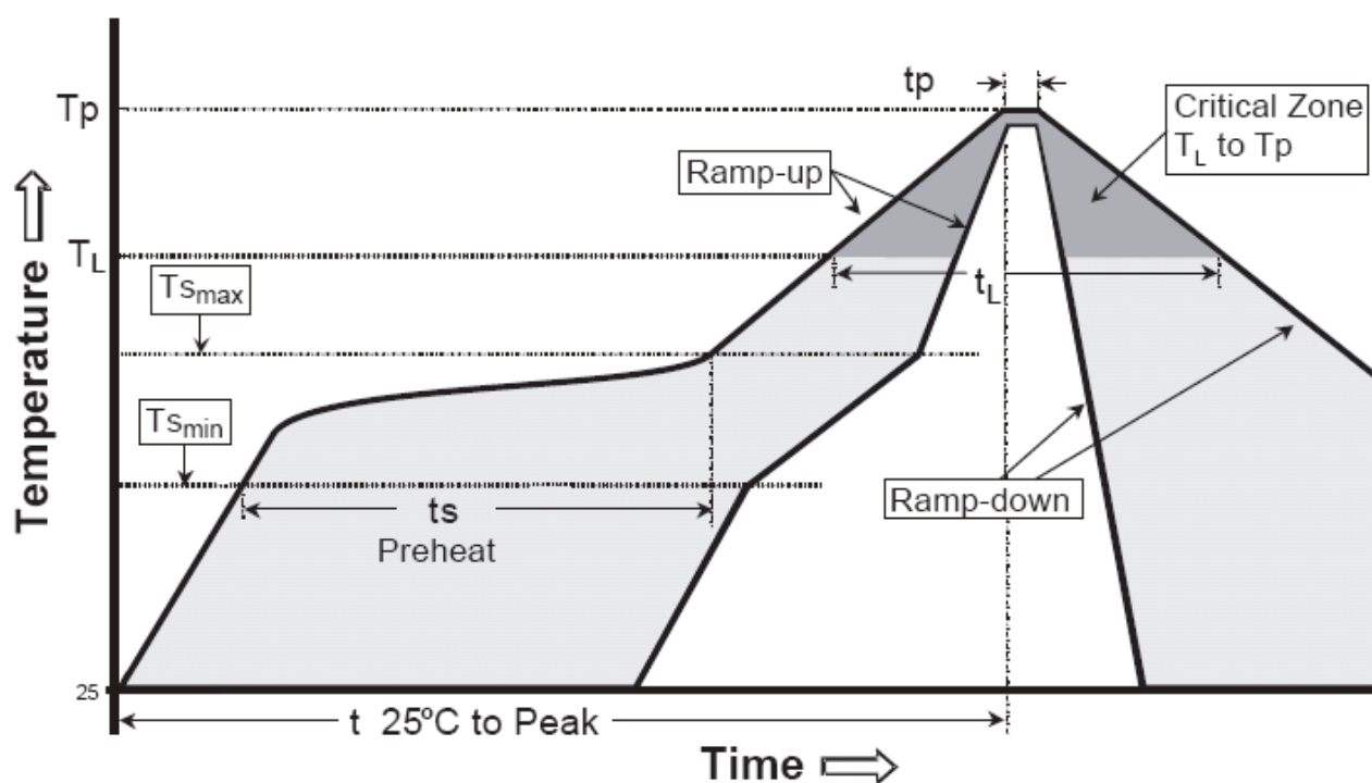
Figure 26-1 Temperature Reflow Profile
