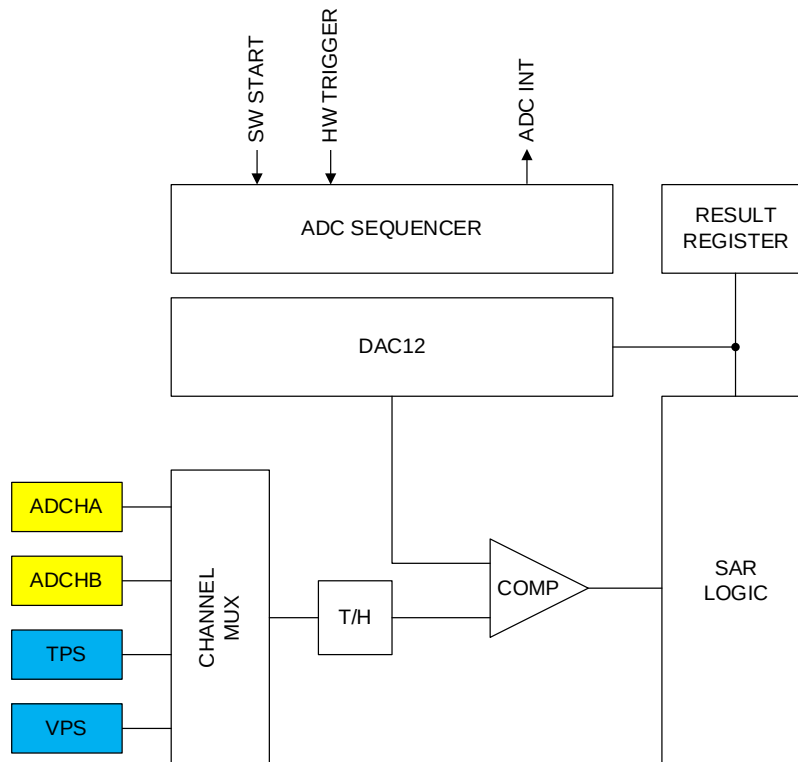
Figure 17-1 12-bit SAR ADC block diagram
