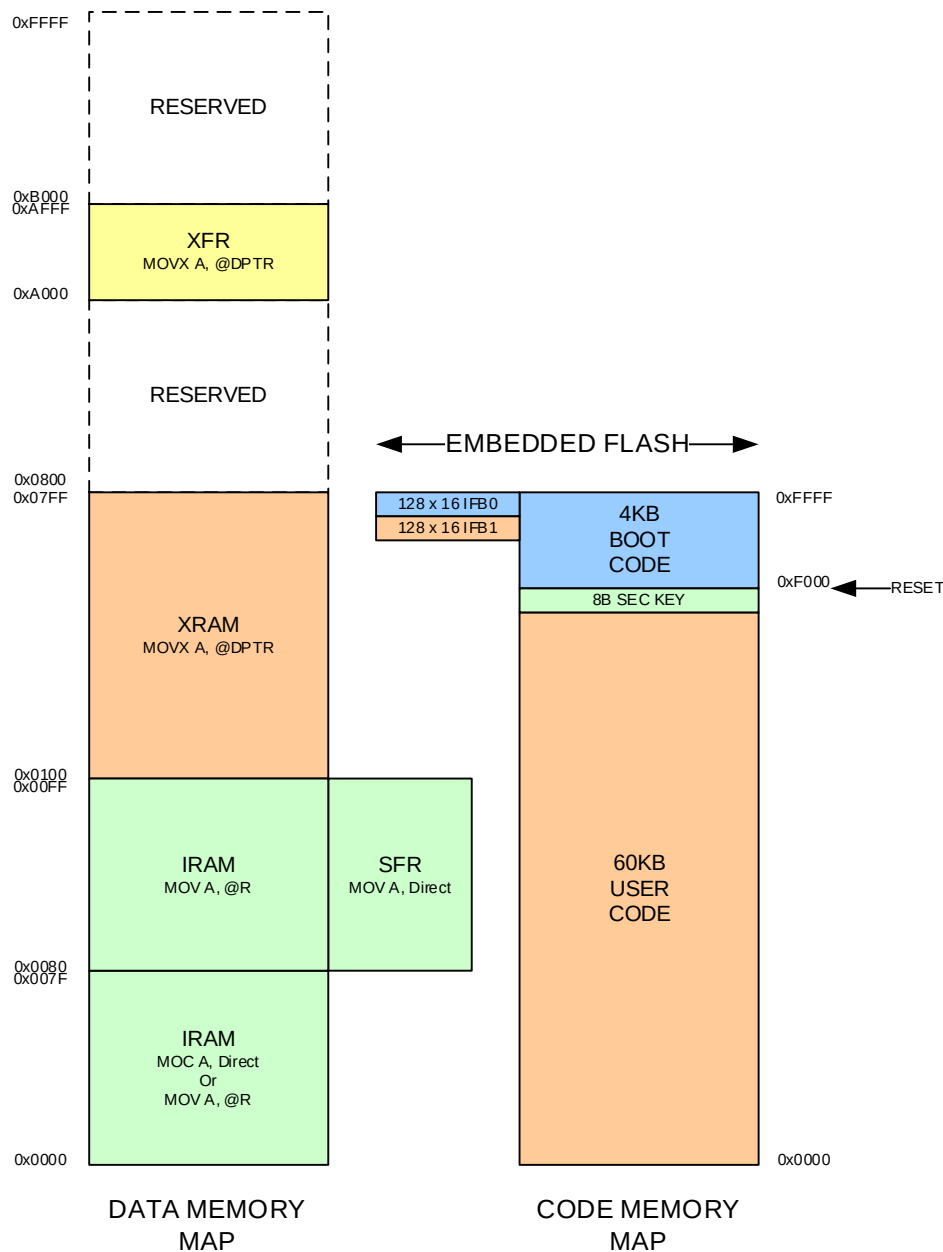
Figure 2-1 Memory Map
