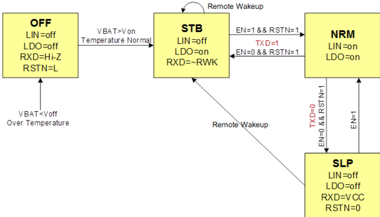
Figure 22-1 LIN State Operation Diagram
