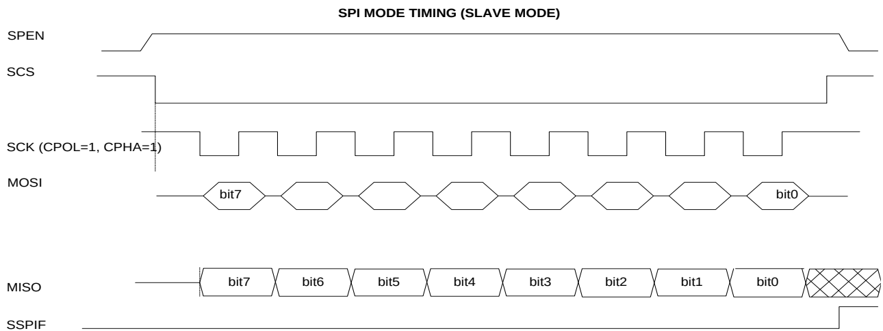
Figure 10-8 SPI Slave Timing with CPOL=1, CPHA=1
