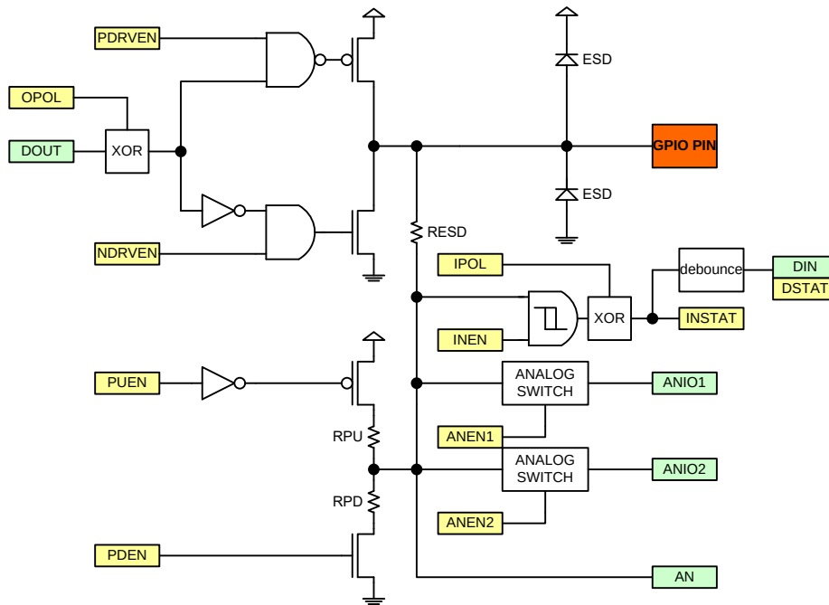
Figure 21-1 GPIO Multi-Function Select and Pin Interrupt
