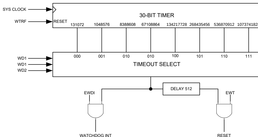
Figure 5-1 Watchdog Time block diagram
