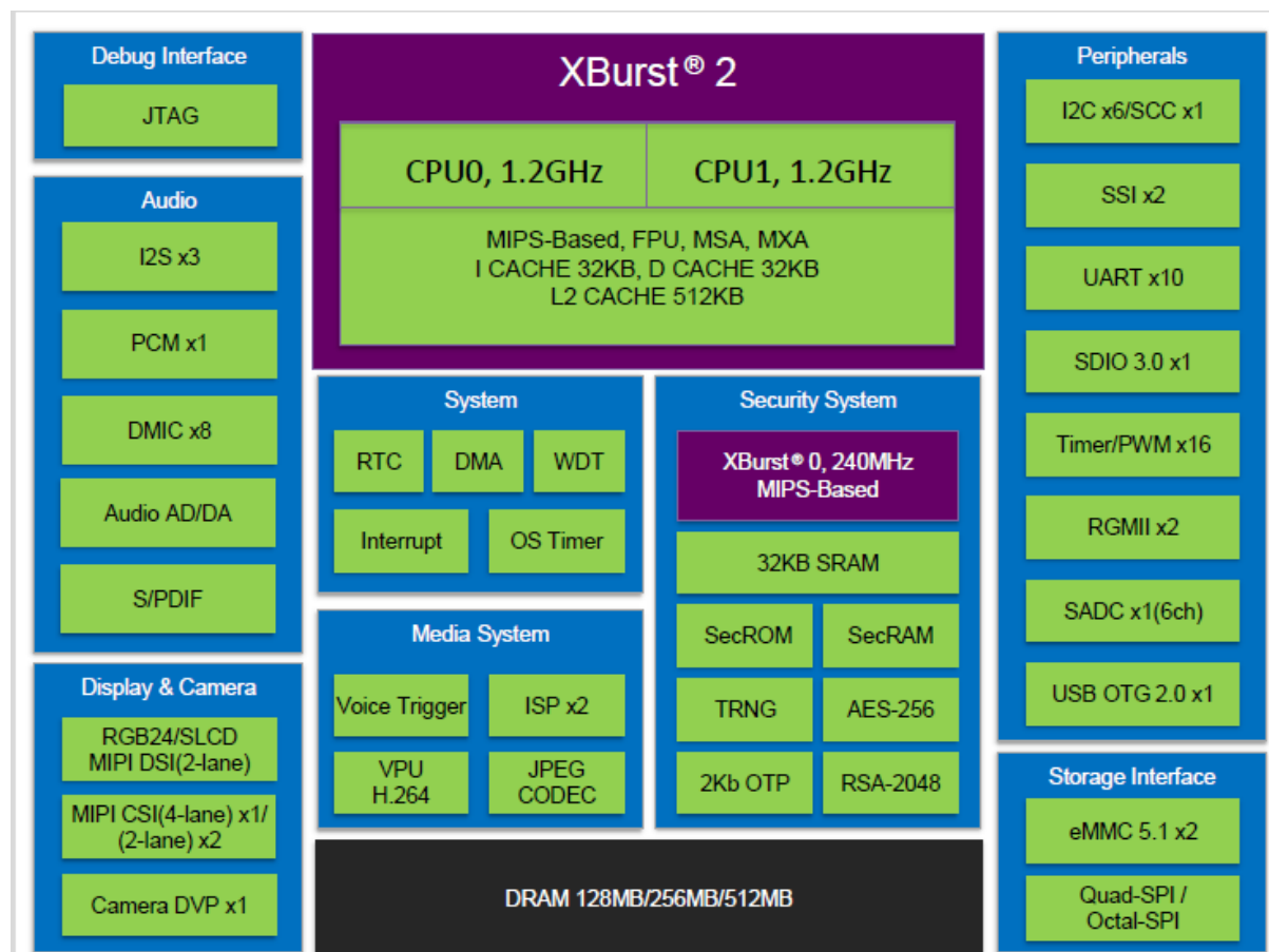
Figure 1-1 X2000/E/H Diagram
