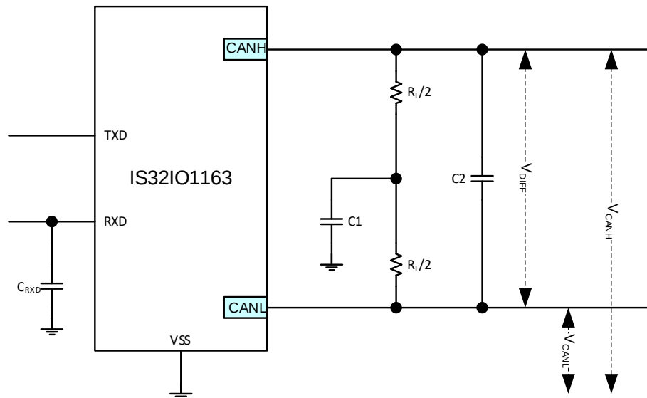
Figure 3-4 HS-PMA test circuit
