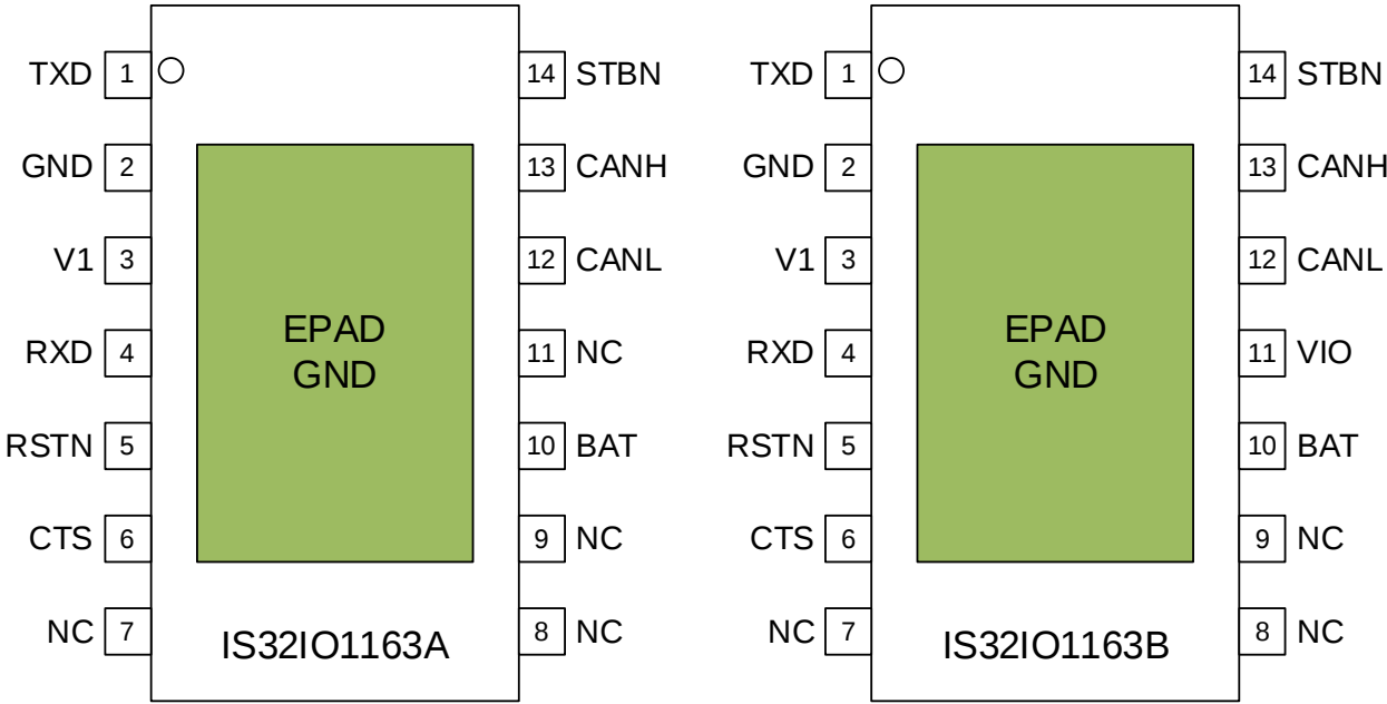
TOP VIEW
