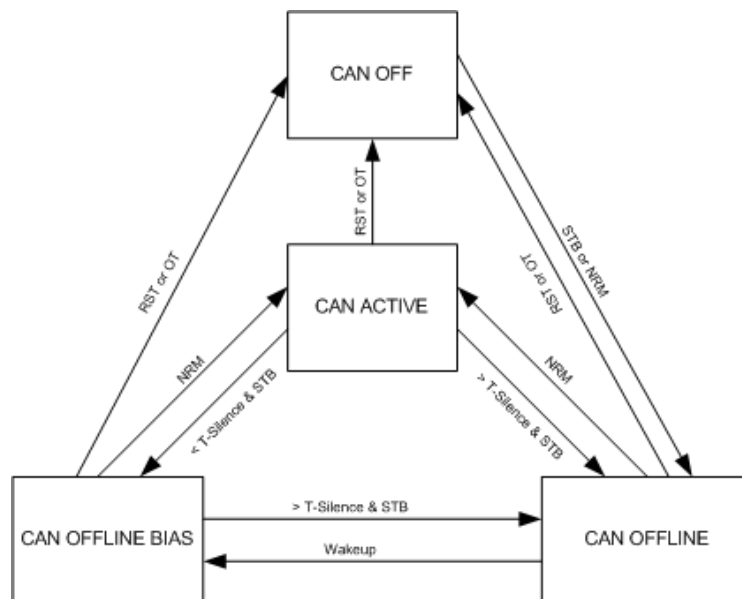
Figure 3-2 CAN transceiver state machine
