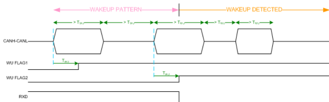
Figure 3-3 CAN wake-up timing
