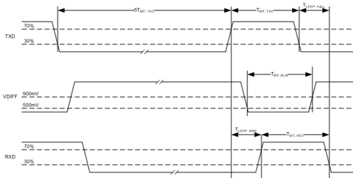
Figure 3-5 HS-PMA implementation timing diagram
