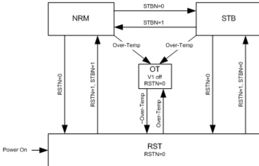
Figure 3-1 System controller state diagram
