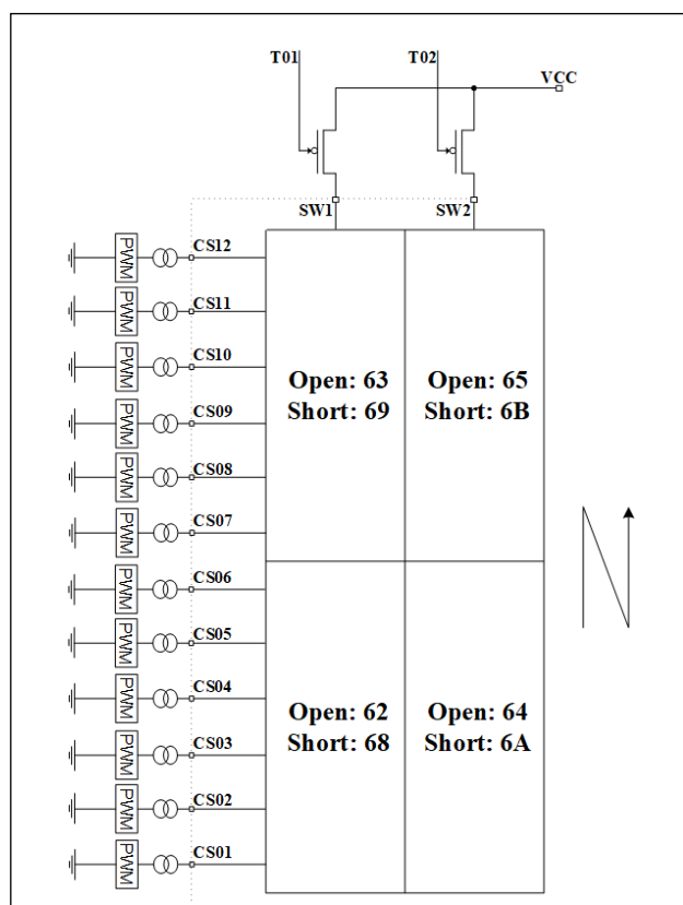
Figure 10 PWM Register
