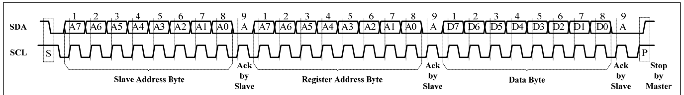
Figure 5 I2C Writing to IS31FL3752 (Typical)
