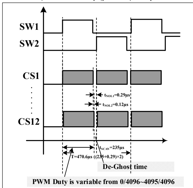
Figure 11 Scanning Timing
