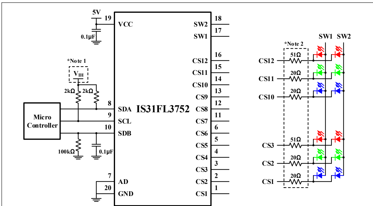
Figure 1 Typical Application Circuit: 12×2, 8 RGBs
