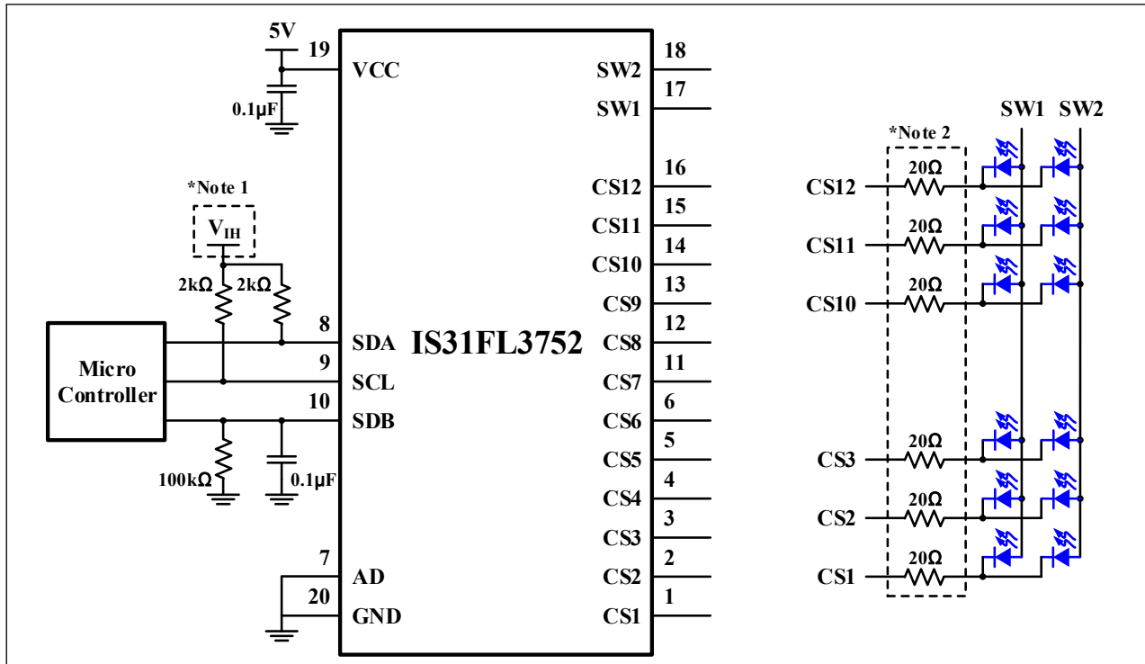
Figure 2 Typical Application Circuit: 24 Mono Color LEDs
