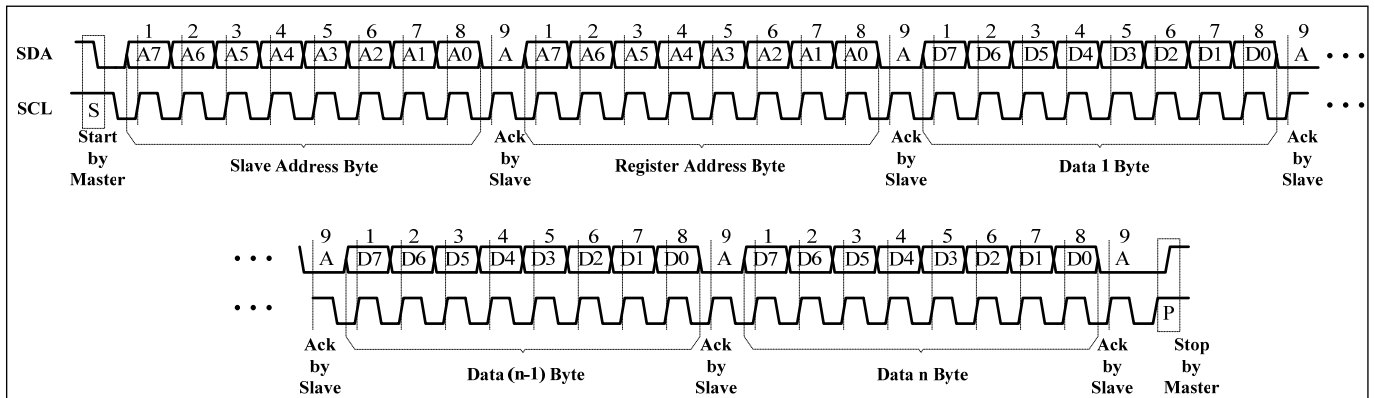
Figure 6 I2C Writing to IS31FL3752 (Automatic Address Increment)
