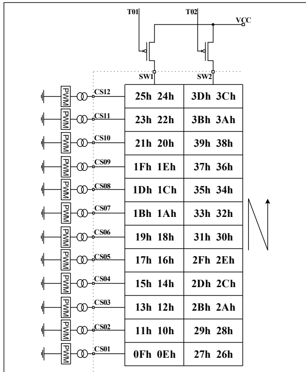
Figure 9 PWM Register
