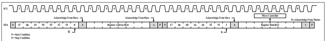
Figure 7 I2C Reading from IS31FL3752
