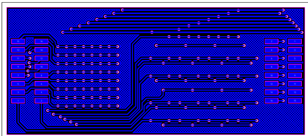
Figure 12: LED Board PCB Layout - Bottom Layer
