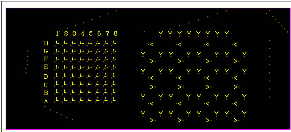
Figure 9: LED Board Component Placement Guide - Top Layer
