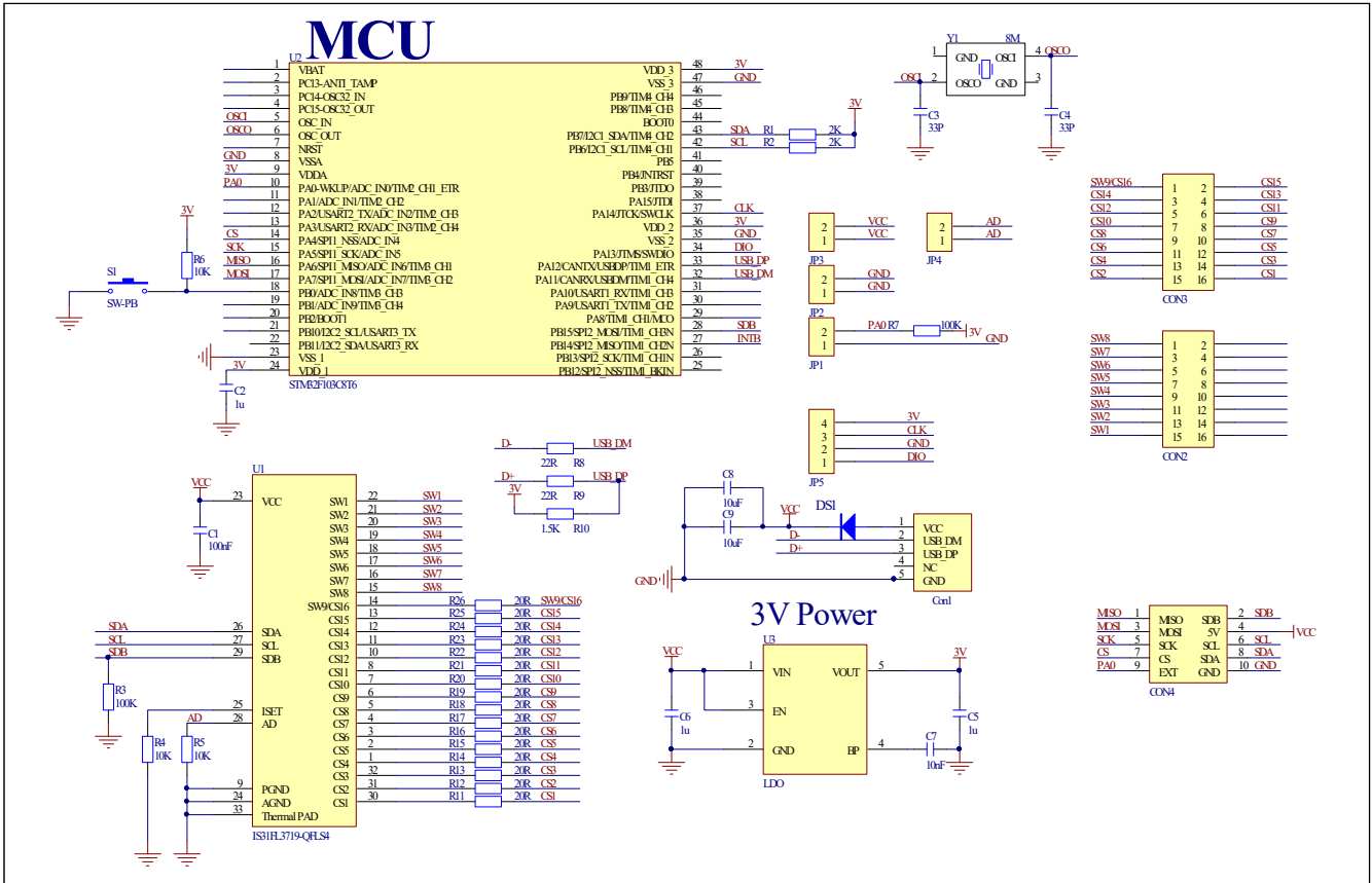
Figure 3: IS31FL3719-QFLS4 Application Schematic
