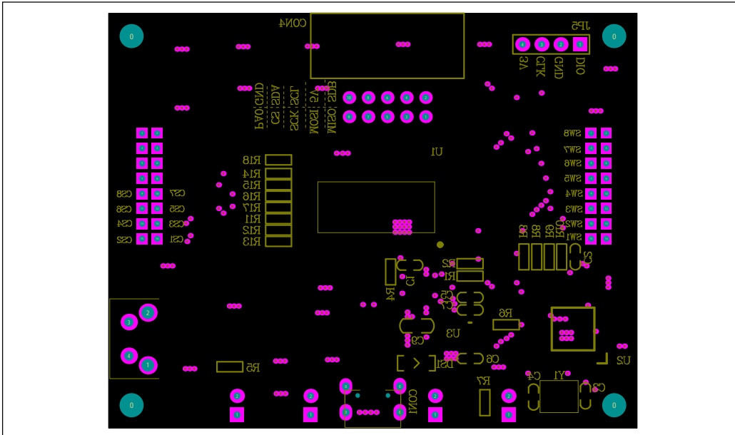
Figure 7: Board Component Placement Guide - Bottom Layer
