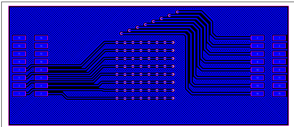
Figure 12: LED Board PCB Layout - Bottom Layer
