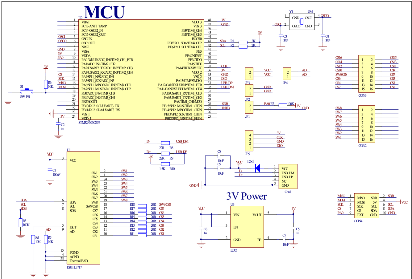
Figure 3: IS31FL3717 Application Schematic
